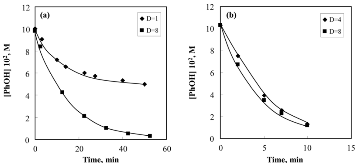
Fig. 4. Theoretical (—) and experimental (◆, ■) profiles of phenol degradation for different oxidant dose D. (a) added [\text{Fe}^{2+}] 3.5 \cdot 10^{-5} M. (b) added [\text{Fe}^{2+}] 9 \cdot 10^{-5} M.
